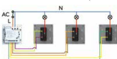
Connection 4: With neutral wire Connect to a Yoswit and other brands 2 way switch.
