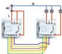
Connection 3: Without neutral wire Connect to a Yoswit and other brands 2 way switch.
