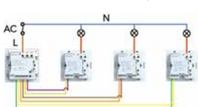
Connection 5: Without neutral wire Connect to a Yoswit and other brands 2 way switch.
