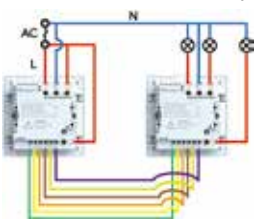
Connection 4: With neutral wire Connect to a Yoswit and other brands 2 way switch.
