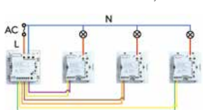
Connection 6: With neutral wire Connect to a Yoswit and other brands 2 way switch.
